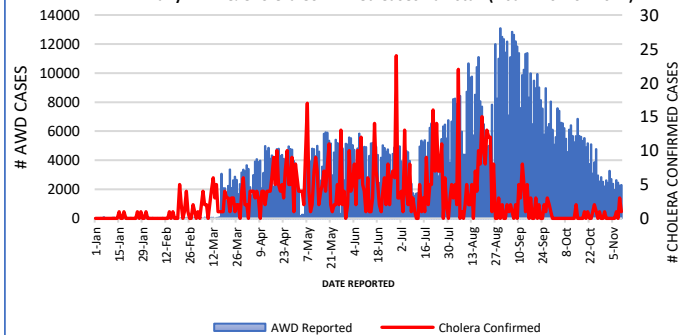
Daily AWD & Cholera Confirmed Cases Pakistan (1 Jan - 10 Nov 2022)
