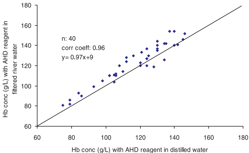
Figure 6b Correlation of haemoglobin (AHD 575 method) in double distilled and filtered river water
