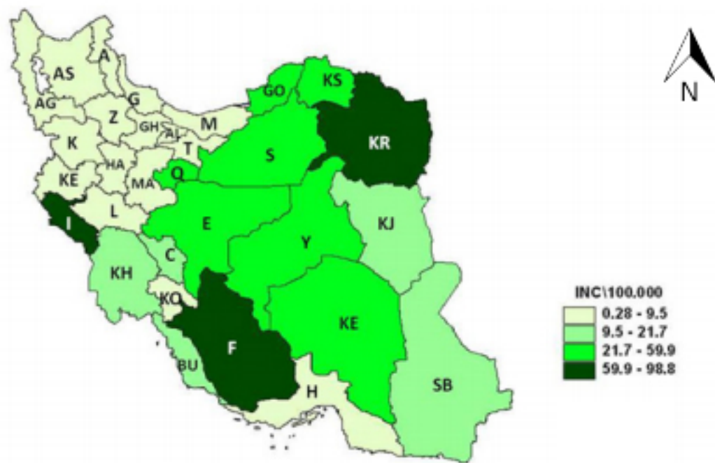
Figure 2 Distribution of incidence of cutaneous leishmaniasis (zoonotic and anthroponotic) in each province of the Islamic Republic of Iran, 2012 (A = Ardabil, AS = East Azerbaijan, AG = West Azerbaijan, T = Tehran, G = Gilan, K = Kordestan, Q = Qom, KS = Khorasan Shomali, KR = Khorasan Razavi, C = Chaharmahal & Bakhtiari, L = Lorestan, KH = Khuzestan, KO = Kohgiluyeh & Boyer-Ahmad, SB = Sistan & Baluchistan, E = Isfahan, F = Fars, S = Semnan, KE = Kerman, KJ = South Khorasan, Y = Yazd, H = Hormozgan, M = Mazandaran, AL = Alborz, GH = Ghazvin, Z = Zanjan, MA = Mazandaran, KE = Kerman, I = Ilam, GO = Golestan, BU = Bushehr, HA = Hamedan)
