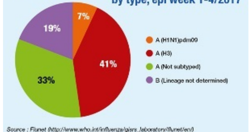
Figure 2. Circulating Influenza viruses in the EMR by type, epi week 1-4/2017
