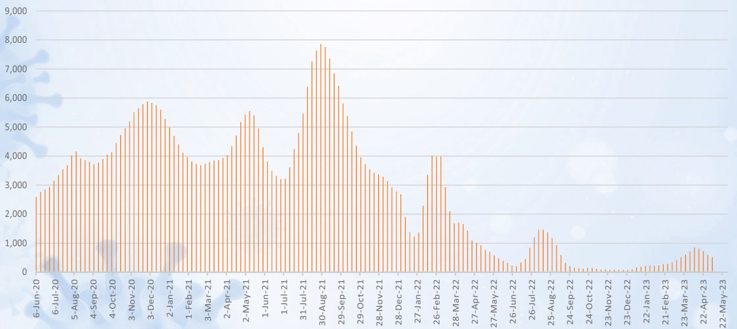
Figure 2. Weekly Trend of COVID-19 Cases in ICU, 06 June 2020-06 May 2023
