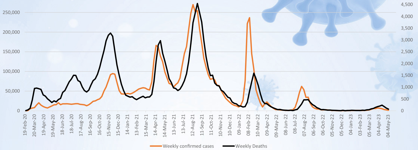
Figure 1. Weekly Trend of COVID-19 Laboratory-Confirmed Cases and Deaths, 19 February 2020 - 06 May 2023
