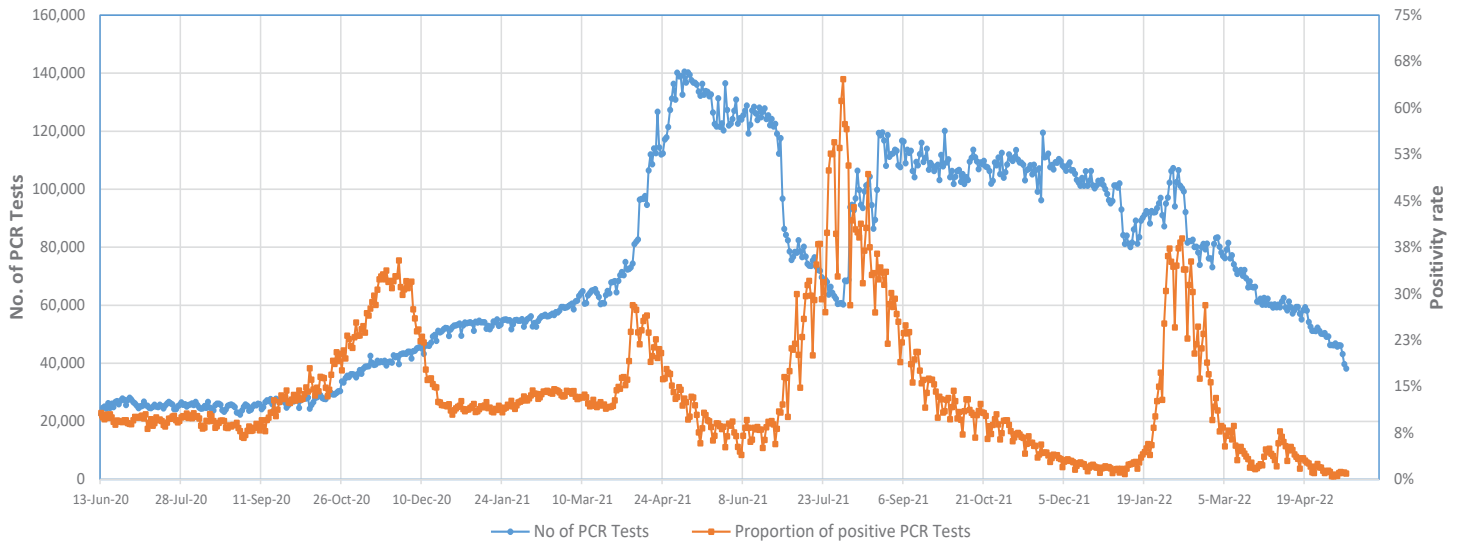
Figure 3 - Number of Daily COVID-19 PCR Tests and Percentage of Positive Cases, 13 April 2020 - 12 May 2022
