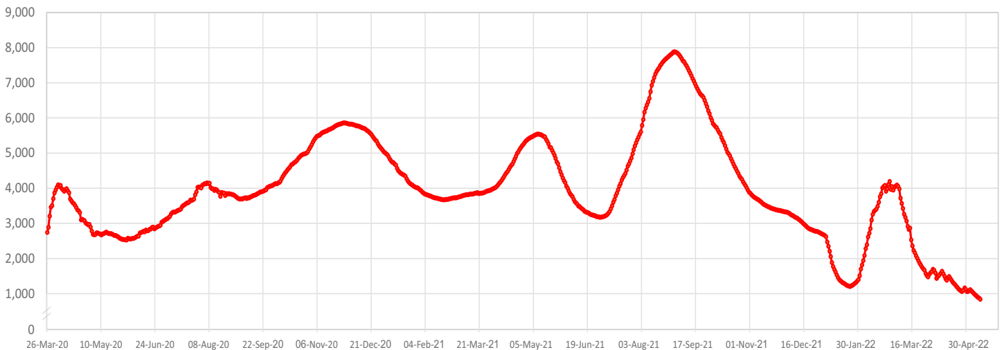
Figure 2 - COVID-19 Patients in Intensive Care, 26 March 2020 - 12 May 2022
