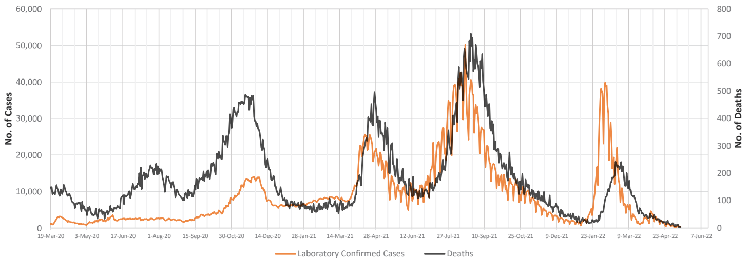
Figure 1 - Trend of COVID-19 Laboratory-Confirmed Cases and Deaths, 19 February 2020 - 12 May 2022
