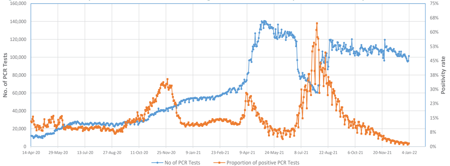
Figure 3 - Number of Daily COVID-19 PCR Tests and Percentage of Positive Cases, 13 April 2020 - 03 January 2022
