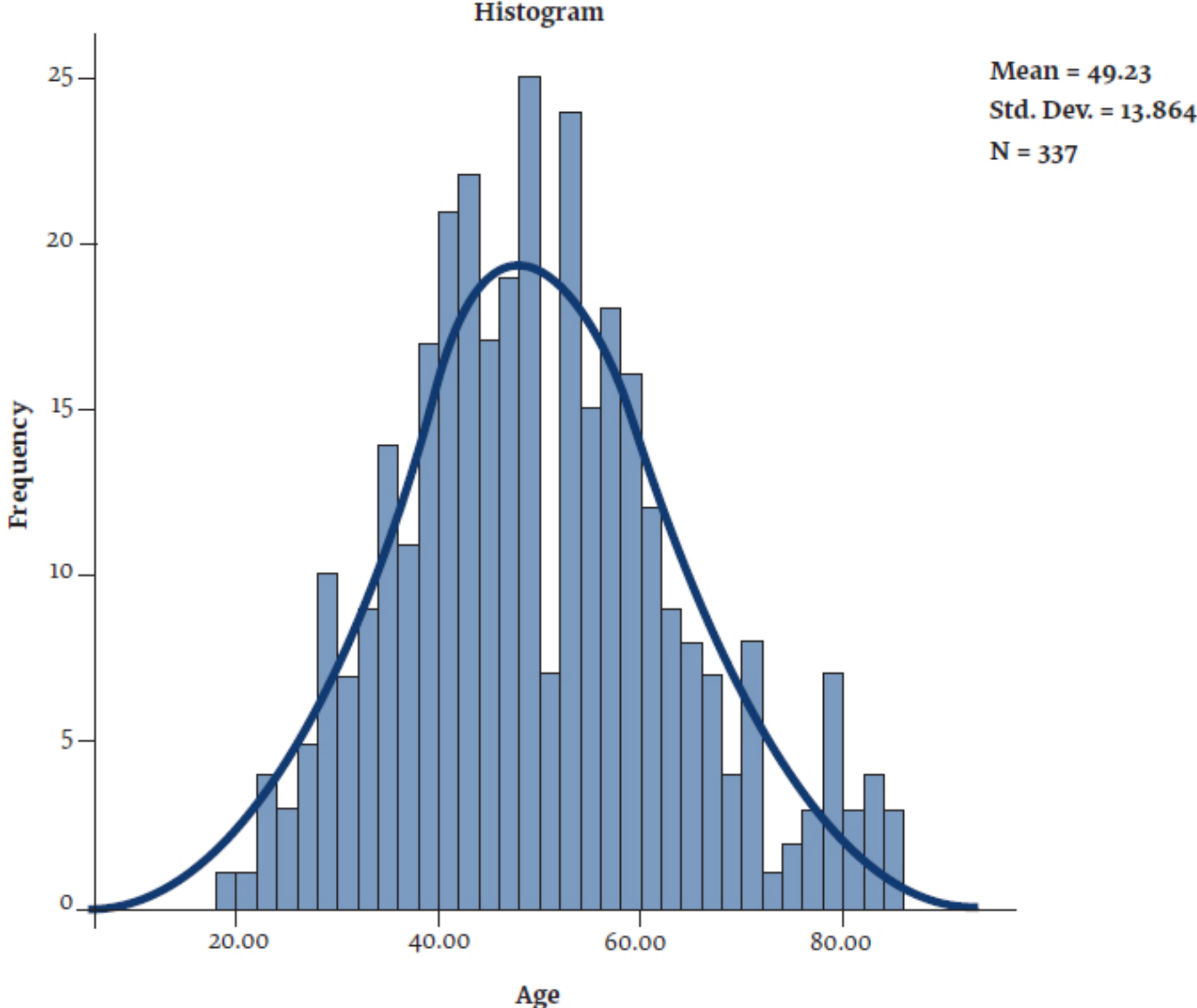
Figure 1 Normal distribution of sample
