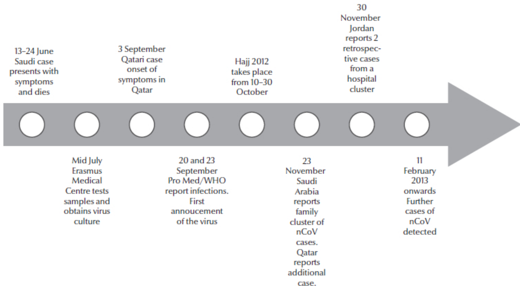
Figure 2 Timeline of novel coronavirus (nCoV) infections
